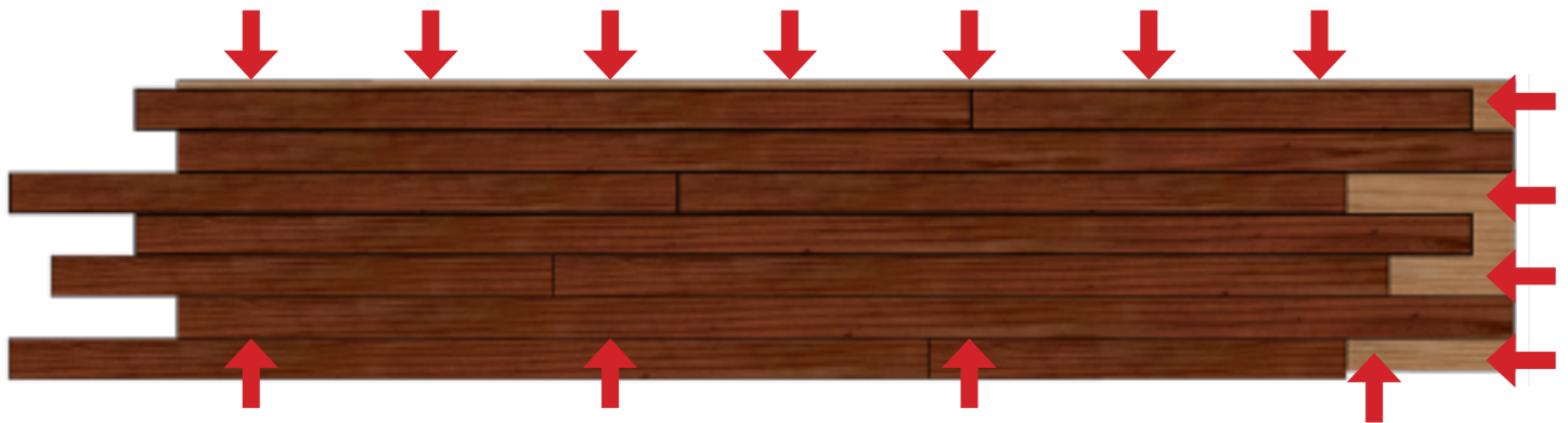
Plank Modular Panel: Nailing Schedule
