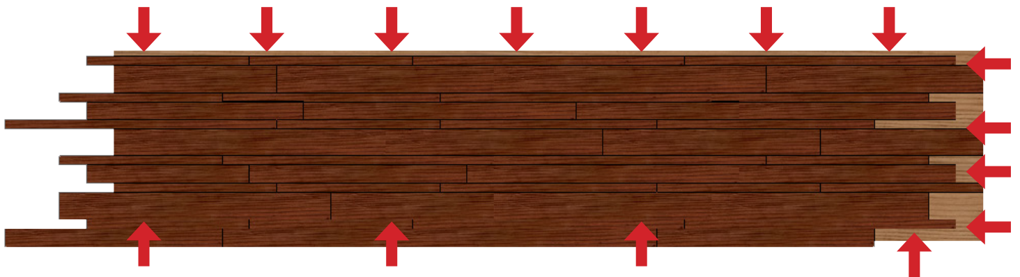
Figure 5 3D Stick Modular Panel: Nailing Schedule
