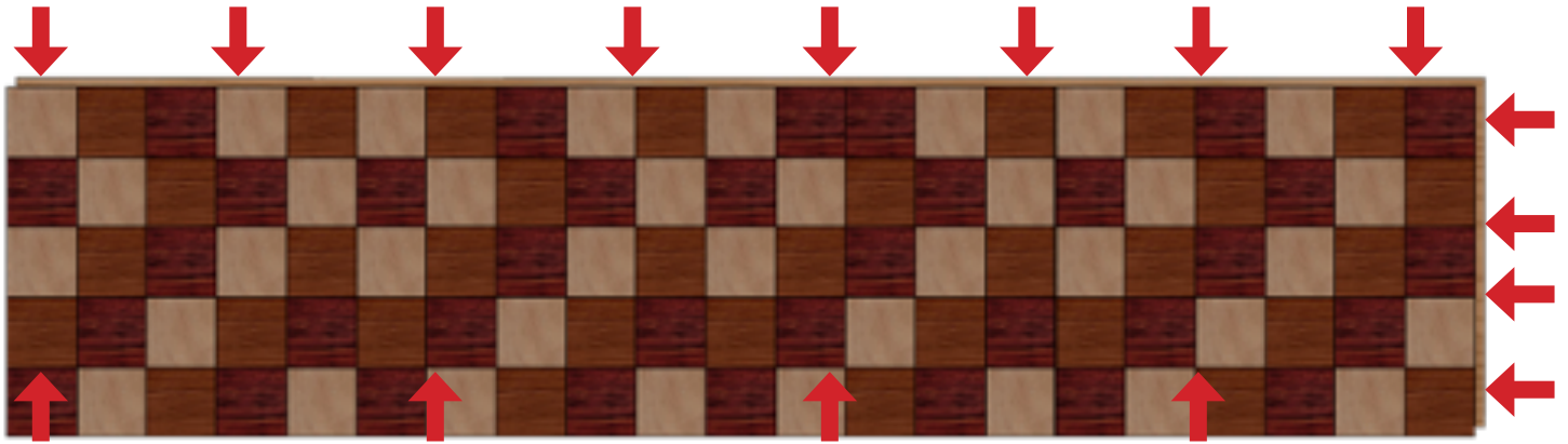
Figure 3 3D Cube Modular Panel: Nailing Schedule
